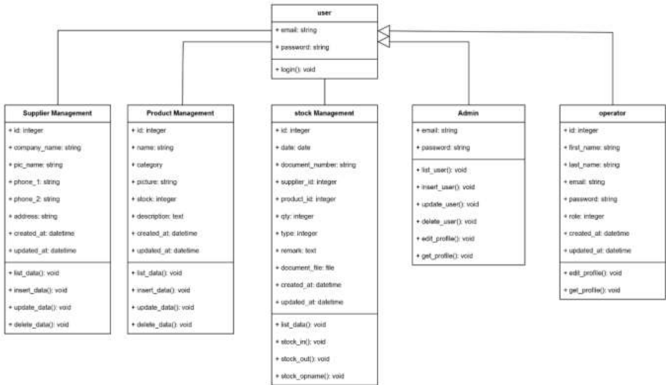
Figure 3. Class diagram
