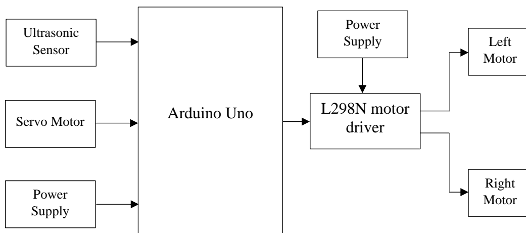
Figure 1. Structure of obstacle avoiding robot
