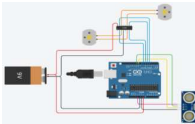
Figure 2: Obstacle avoiding robot circuit diagram
