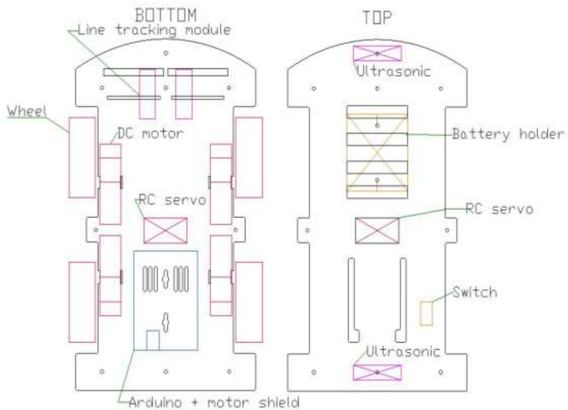
Figure 3. Robotic vehicle chassis design
