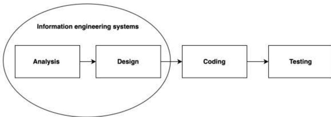
Figure 1. Waterfall model [6]
