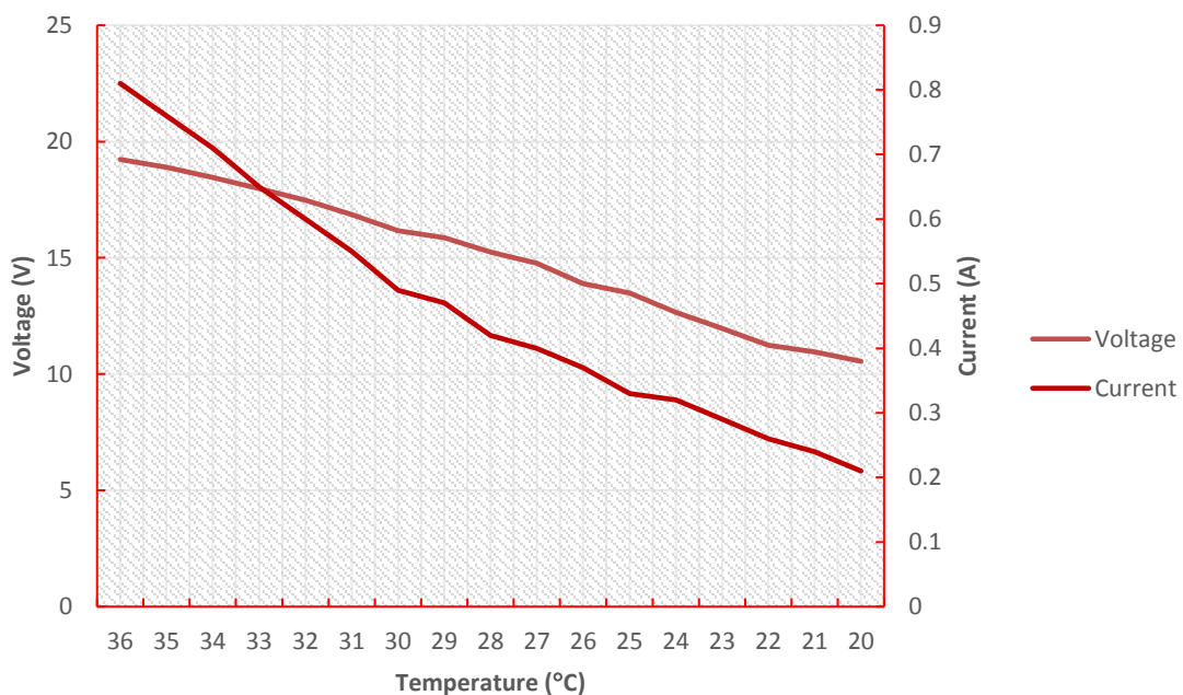
Figure 3. Solar panel test
