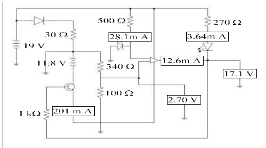
Figure 2 (b). 12V battery charging circuit diagram
