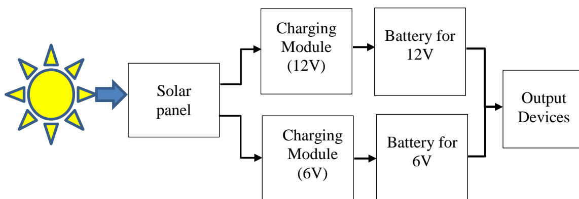
Figure 1. Structure of power system
