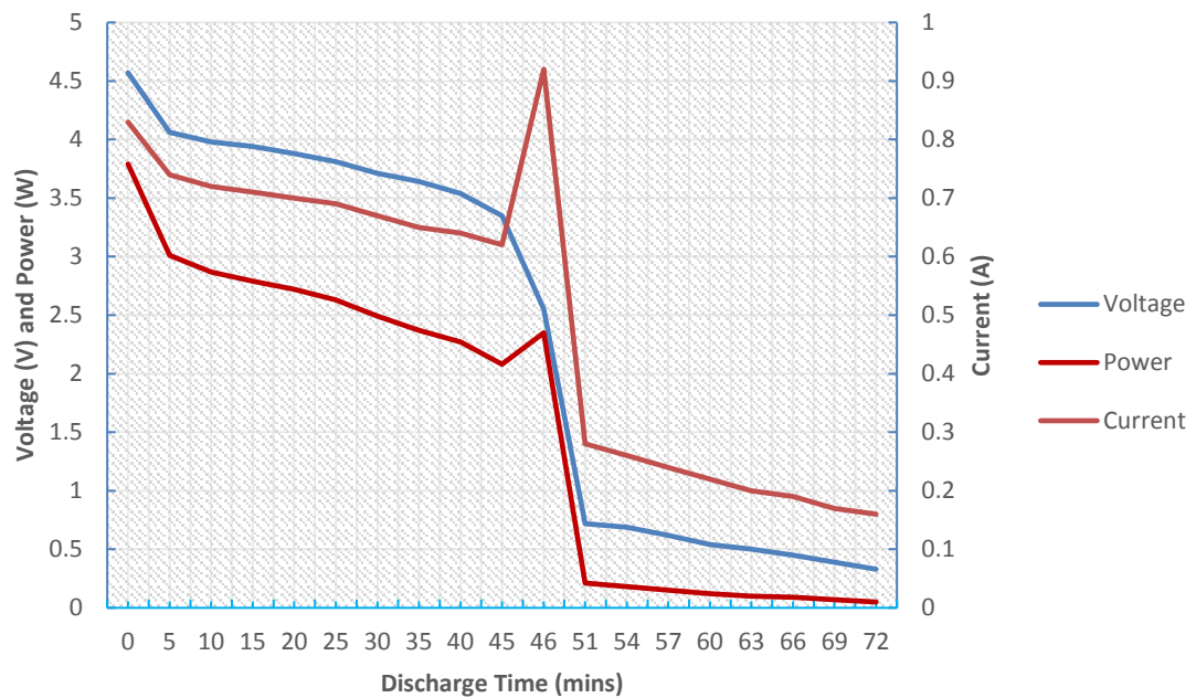
Figure 5. Discharge of Manganese Dioxide Battery
