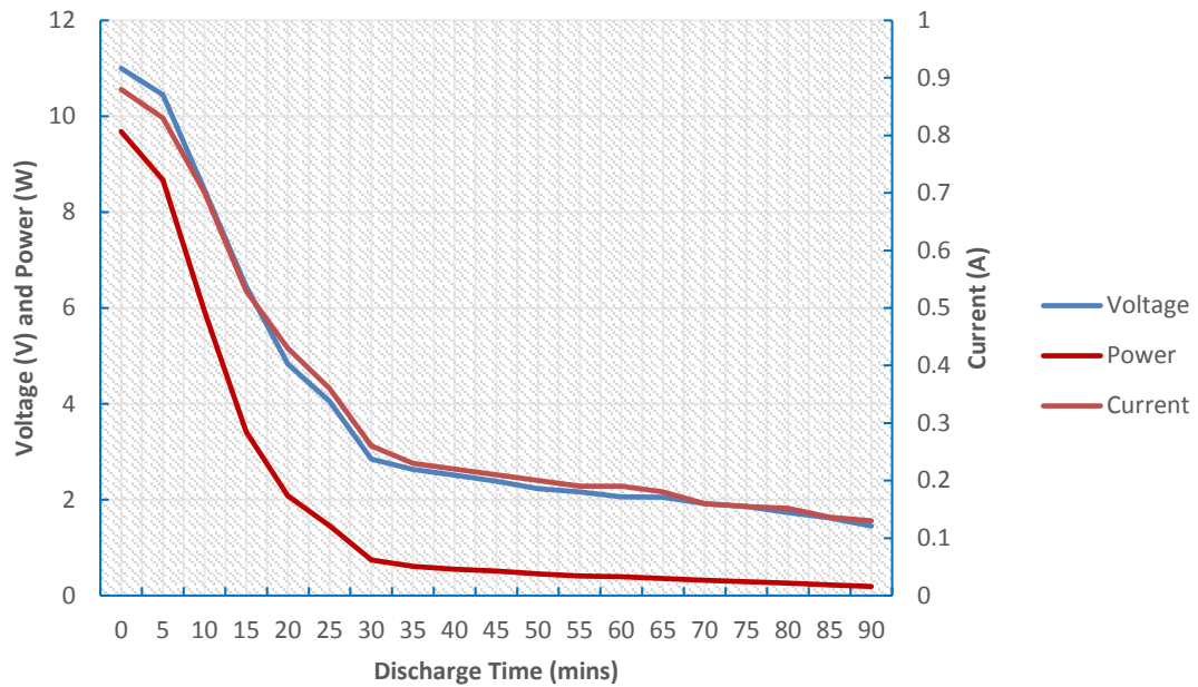
Figure 4. Discharge of Lead Acid Battery
