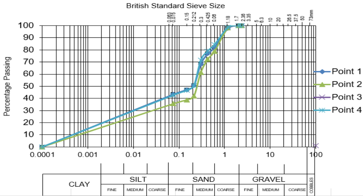
Figure 3: Sieve Analysis Graph of Soil Samples
